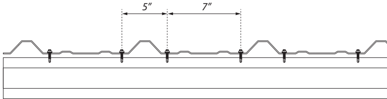
FASTENER PATTERN 5"–7"–5" (over steel purlin)
